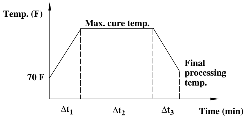
FIGURE 4. THE TEMPERATURE CYCLE USED FOR CURING THE BASE LAMINATE AND IN MAKING THE REPAIR
