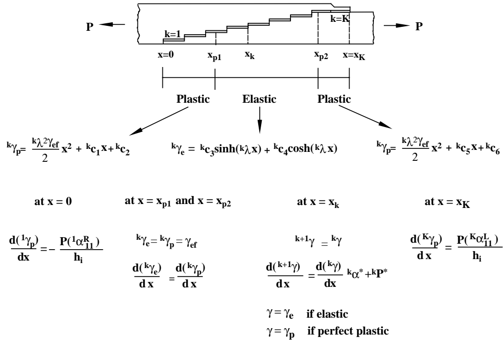
FIGURE 58. THE EQUATIONS AND BOUNDARY AND CONTINUITY CONDITIONS FOR CALCULATING THE SHEAR STRAIN IN THE INTERLAYER WHEN THE INTERLAYER IS PERFECTLY PLASTIC NEAR THE x = 0 AND x = x_K ENDS
