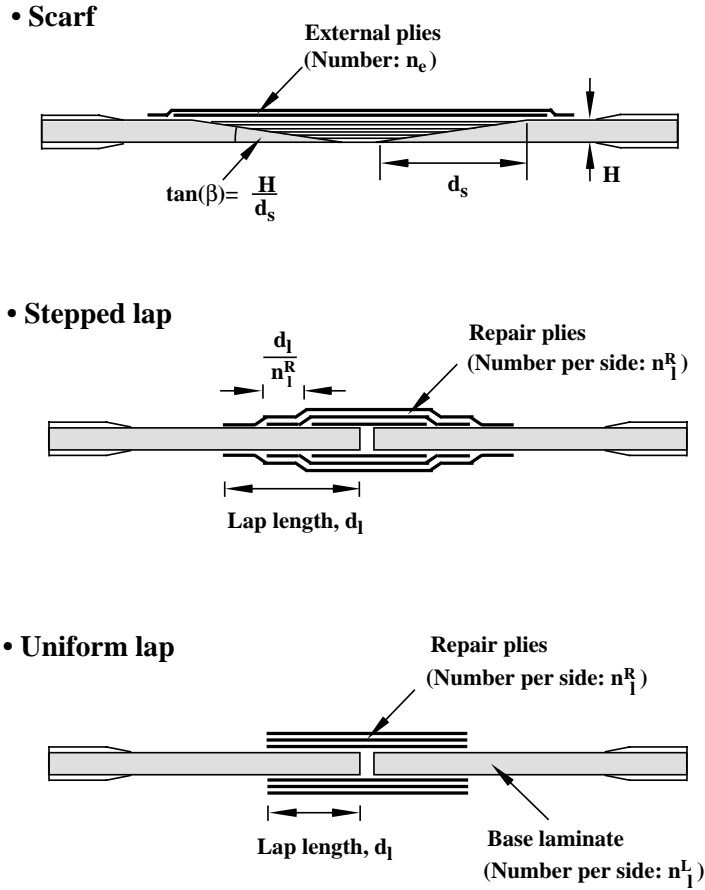
FIGURE 14. DEFINITION OF THE GEOMETRIC FACTORS INVESTIGATED
