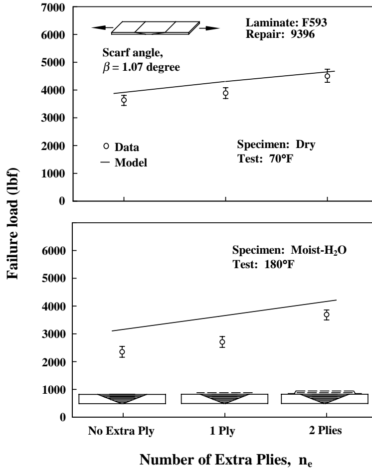
FIGURE 62. COMPARISON OF THE CALCULATED (MODEL) AND THE MEASURED (DATA) FAILURE LOADS AS A FUNCTION OF EXTRA PLYS
