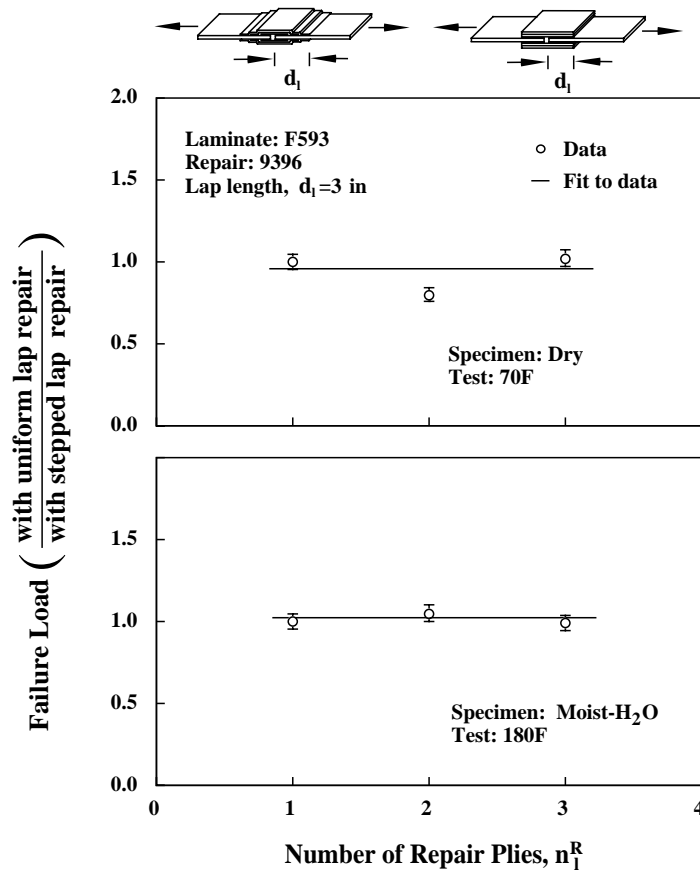
FIGURE 21. COMPARISONS OF THE FAILURE LOADS OF SPECIMENS REPAIRED BY THE STEPPED LAP AND UNIFORM LAP REPAIR TECHNIQUES
