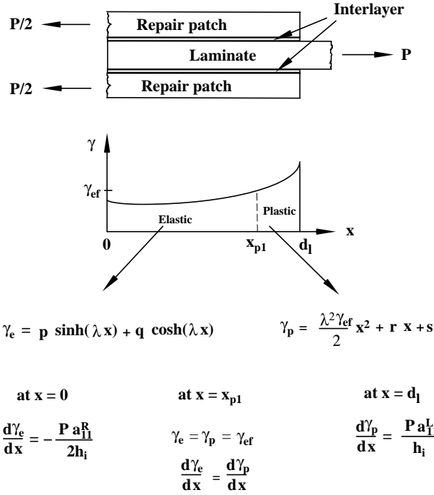
FIGURE 42. THE EQUATIONS AND BOUNDARY AND CONTINUITY CONDITIONS FOR CALCULATING THE SHEAR STRAIN IN THE INTERLAYER WHEN THE INTERLAYER IS PERFECTLY PLASTIC NEAR THE x = d_1 END
