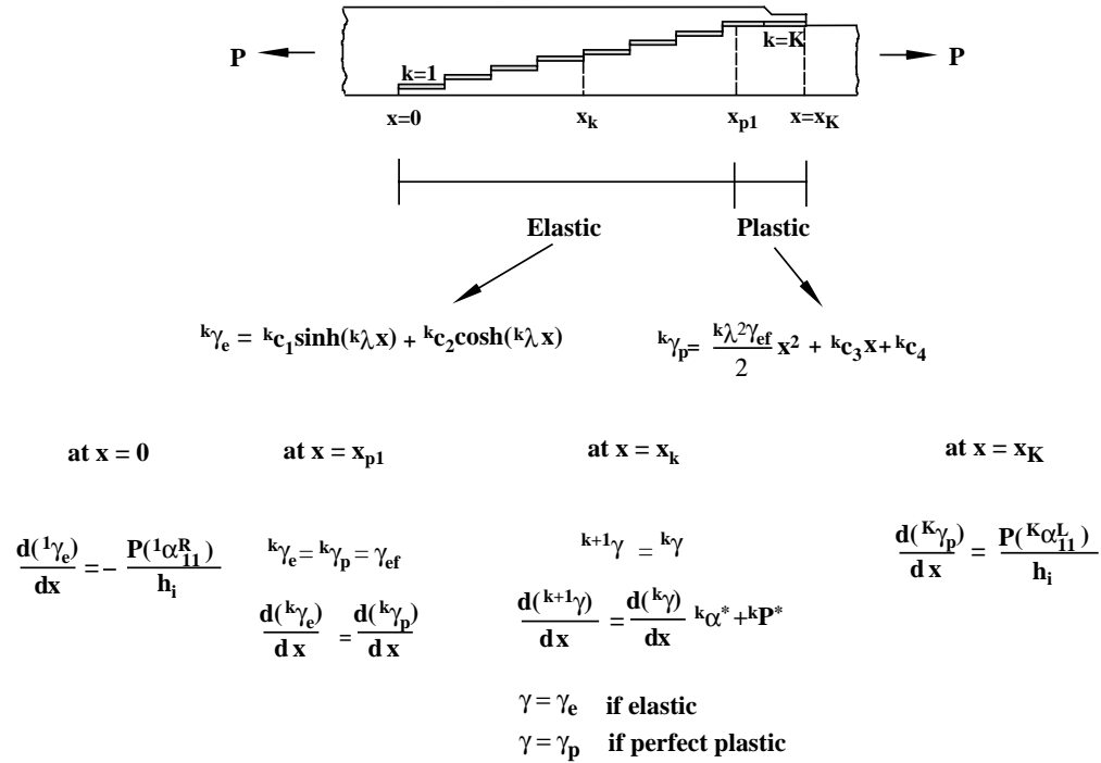
FIGURE 57. THE EQUATIONS AND BOUNDARY AND CONTINUITY CONDITIONS FOR CALCULATING THE SHEAR STRAIN IN THE INTERLAYER WHEN THE INTERLAYER IS PERFECTLY PLASTIC NEAR THE x = x_K END
