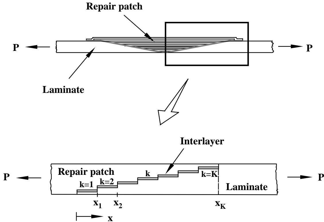
FIGURE 46. THE SCARF REPAIR TREATED IN THE MODEL
