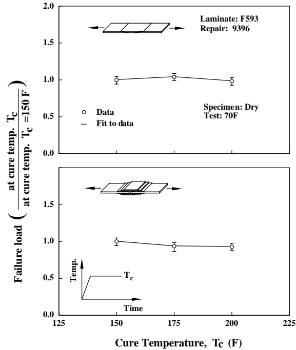
FIGURE 28. FAILURE LOADS OF SPECIMENS REPAIRED AT DIFFERENT CURE TEMPERATURES (Specimen geometries are given in figures 5 and 14. Failure loads of the specimens at cure temperature 150°F are given in appendix C.)
