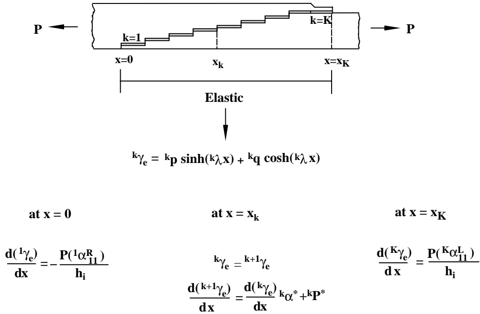
FIGURE 55. THE EQUATIONS AND BOUNDARY CONDITIONS FOR CALCULATING THE SHEAR STRAIN IN THE INTERLAYER WHEN THE ENTIRE INTERLAYER BEHAVES IN A LINEARLY ELASTIC MANNER
