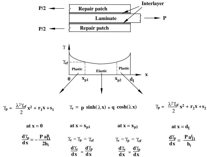
FIGURE 43. THE EQUATIONS AND BOUNDARY AND CONTINUITY CONDITIONS FOR CALCULATING THE SHEAR STRAIN IN THE INTERLAYER WHEN THE INTERLAYER IS PERFECTLY PLASTIC NEAR THE x = 0 AND x = d_1 ENDS
