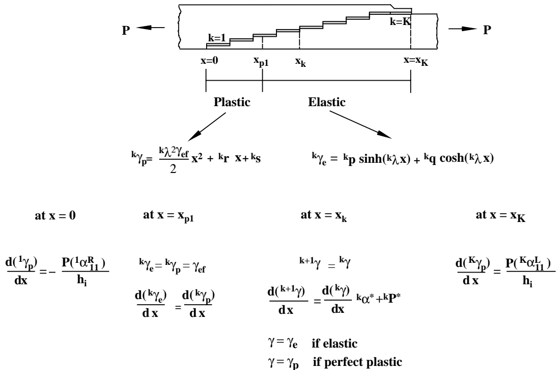
FIGURE 56. THE EQUATIONS AND BOUNDARY AND CONTINUITY CONDITIONS FOR CALCULATING THE SHEAR STRAIN IN THE INTERLAYER WHEN THE INTERLAYER IS PERFECTLY PLASTIC NEAR THE x = 0 END
