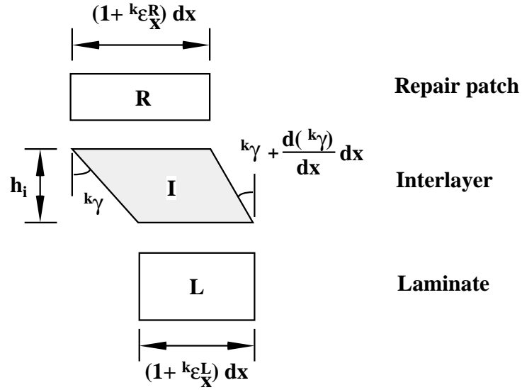
FIGURE 48. DEFORMATIONS OF THE REPAIR PATCH, THE INTERLAYER, AND THE LAMINATE IN THE k -th SEGMENT OF A LAMINATE REPAIRED BY THE SCARF TECHNIQUE
