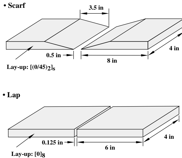
FIGURE 2. THE BASE LAMINATES PRIOR TO REPAIR (Top: laminates used for scarf repair. Bottom: laminates used for lap repair.)
