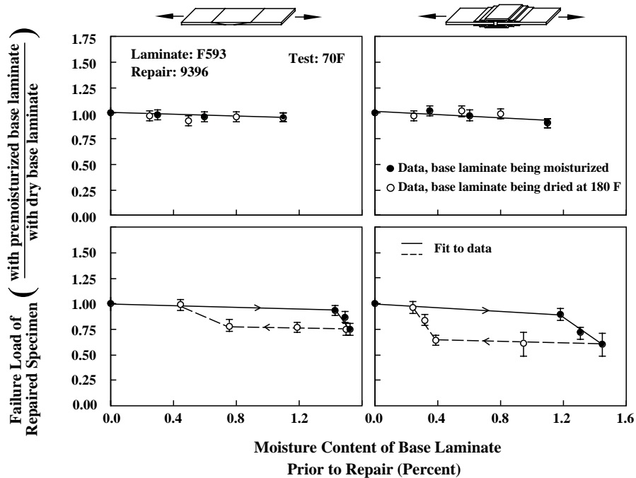
FIGURE 22. FAILURE LOADS OF REPAIRED SPECIMENS WHEN THE BASE LAMINATES WERE MOISTURIZED PRIOR TO REPAIR
