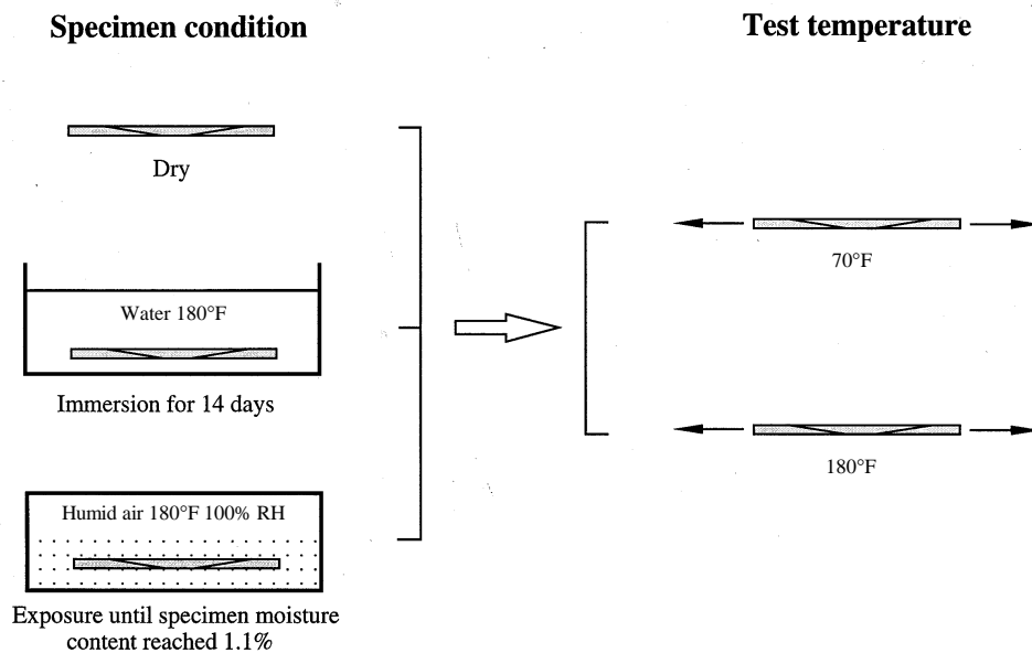
FIGURE 8. SPECIMEN CONDITIONS AND TEST TEMPERATURES
