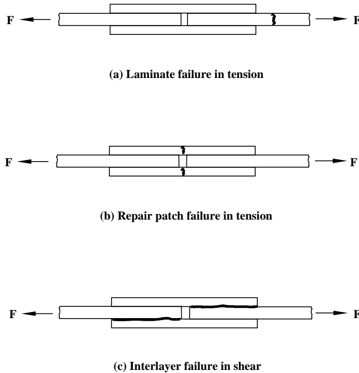
FIGURE 34. ILLUSTRATION OF THE TYPES OF FAILURE WHICH MAY OCCUR IN A LAMINATE REPAIRED BY THE DOUBLE-SIDED UNIFORM LAP TECHNIQUE
