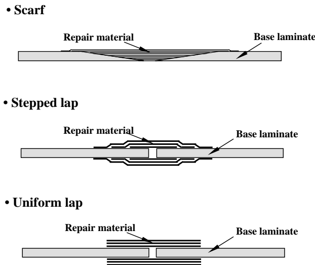
FIGURE 3. ILLUSTRATION OF THE REPAIR TECHNIQUES USED IN THIS STUDY
