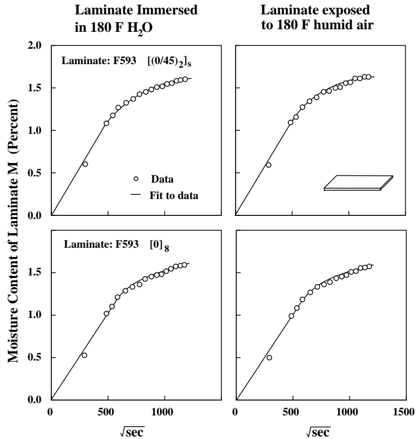
FIGURE A-1. MOISTURE CONTENTS OF THE BASE LAMINATES IMMERSSED IN WATER AT 180°F (LEFT), OR EXPOSED TO 100 PERCENT HUMID AIR AT 180°F (RIGHT)
