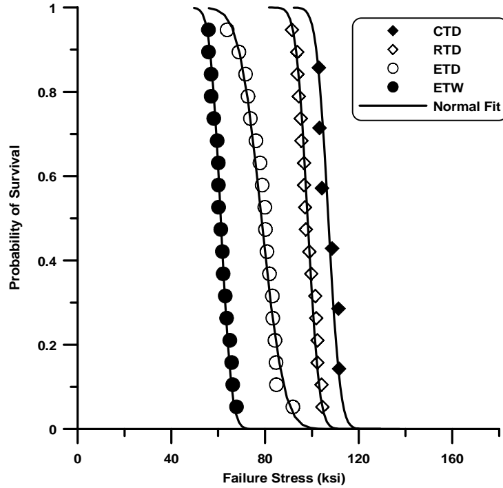
FIGURE 21. NORMALIZED FIT OF EXPERIMENTAL DATA FOR EACH ENVIRONMENT
