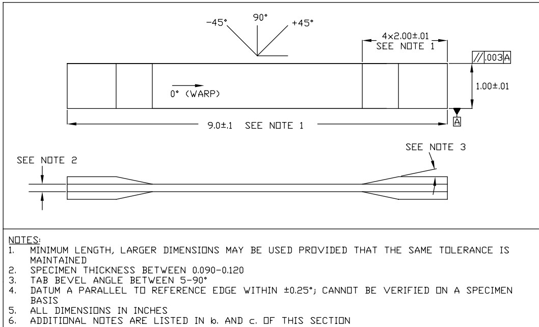
FIGURE 10. ZERO-DEGREE (WARP) WOVEN FABRIC TENSION SPECIMEN
